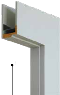
INOVIO frame Invisible frame from our workshop. Specially structured from particleboard designed for plasterboard partitions, allowing the INOVIO frame to completely blend in with its surroundings.
